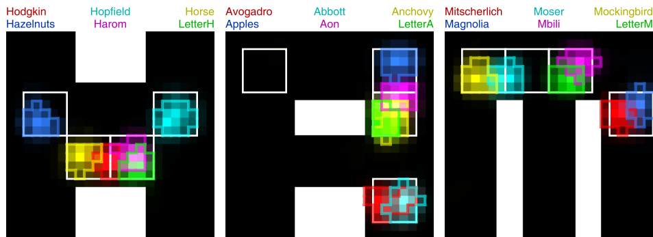
Figure 1.5: Nucleation heatmaps for the indicated training patterns are superimposed on their respective target shapes. The color of an (x, y) location is the RGB sum of adjusted heatmap greylevels (linearly proportional to the spatial nucleation rate \eta_{x,y}^+ for the given shape and pattern, but adjusted for visual clarity) times the given pattern’s indicated color. Colored outlines indicate the smallest region accounting for 75% of nucleation for the given pattern. White square outlines indicate the preferred regions with weighting w_{x,y} = 2 during training.
