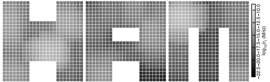
Per-tile nucleation rate: VarHárom4, G_{se}=5.6 , trials=40000
