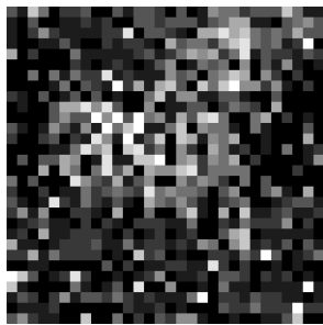
Nucleation model: NoisyHorse3
