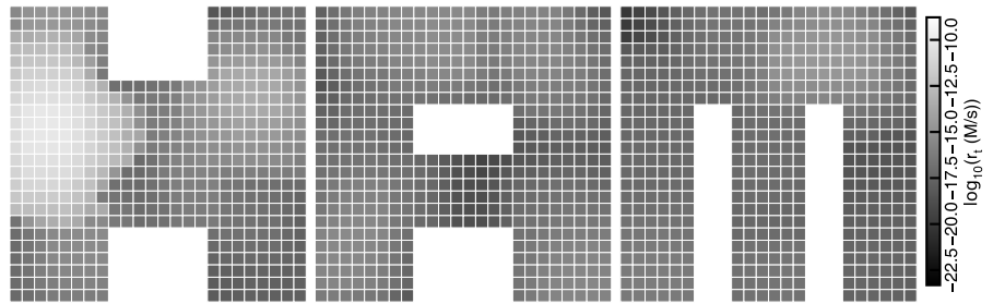
Per-tile nucleation rate: ObscHazeln1, G_{se}=5.6 , trials=40000
