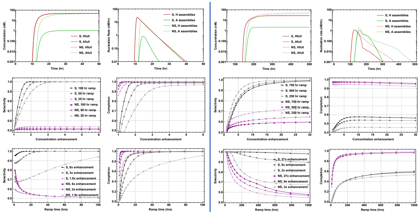
Figure 1.4: Simulation results examining the winner-take-all effect due to depletion during an anneal. The CG model is shown on the left, and the SGM-lite CRN model is shown on the right. All simulations were done with a base concentration of 50 nM. The top plots show concentrations of complete assemblies and nucleation rates as a function of time for an intermediate temperature ramp rate (50 hours and 500 hours respectively) and an intermediate concentration enhancement (3-fold and 9-fold respectively). In the lower plots, selectivity is computed as the fraction of final complete assemblies that are the target shape, H, and completion is computed as the final concentration of the target shape as a fraction of the limiting base concentration. Nucleation is computed as the rate of production of H_{nuc} or A_{nuc} in the CG model, and as the net rate of production of assemblies containing at least 25 tiles in the SGM-lite model.
