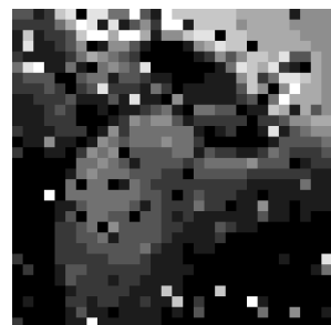
Nucleation model: NoisyApple1
