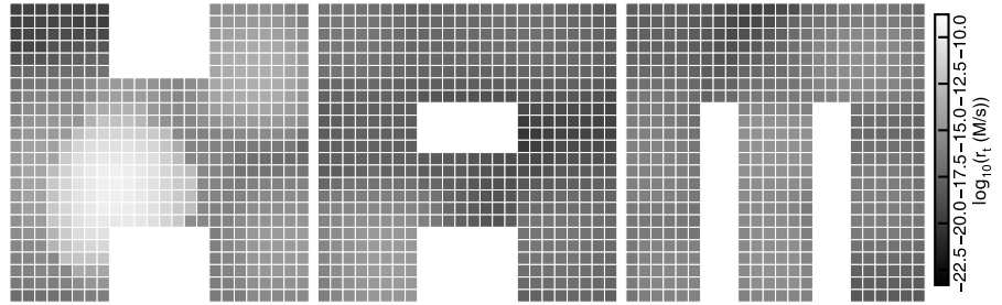
Per-tile nucleation rate: NoisyHorse3, G_{se}=5.6 , trials=40000
