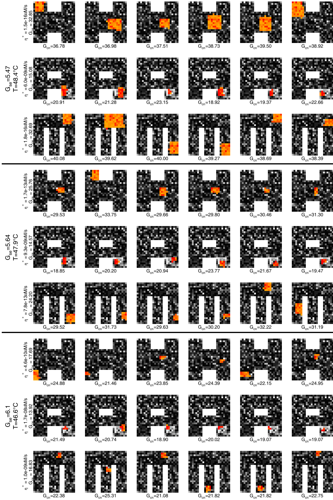
Figure 1.2: A Boltzmann-weighted sample of 6 'critical nuclei' for each shape, at three temperatures, for Avogadro. The color scale from orange to red scales linearly from the lowest to highest concentration, and is used for tiles that are part of the critical nucleus; the color scale from black to white is used analogously for tiles not in the nucleus. \eta^+ is the estimated nucleation rate for the shape; G_{ce} is the corresponding critical nucleus ensemble free energy; G_{se} is per-bond differential sticky-end energy at the shown temperature; and G_{cn} is the chemical potential of the given critical nucleus.
