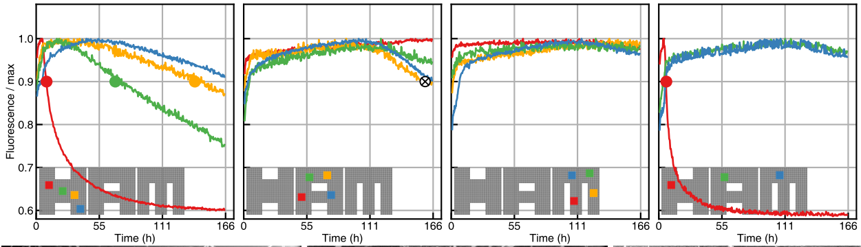
Pattern recognition ramp: Hazelnuts
