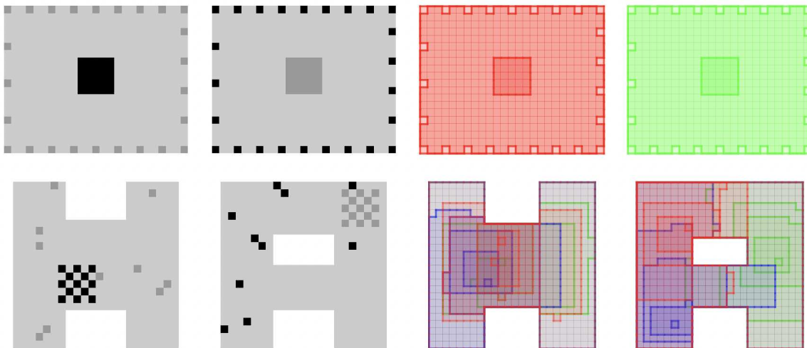
Figure 1.3: Schematic illustration of the CG CRN model (top) and the SGM-lite CRN model (bottom). On the left are the two shapes, called “H” and “A”, with black indicating the set of tiles whose concentrations will be enhanced in this study to favor nucleation of H, and intermediate grey indicating another set of tiles that could be used to favor nucleation of A. On the right we indicate the assemblies that are considered in the models: The CG CRN just uses three assemblies for each shape, e.g. H_{nuc} , H_{mid} , and H_{full} . The SGM-lite CRN considers all assemblies that occur in M pre-computed stochastic greedy trajectories for each shape, starting from a single high-concentration tile and proceeding by monomer addition to the full shape. Outlines of sample assemblies along three color-coded trajectories are shown for each shape.
