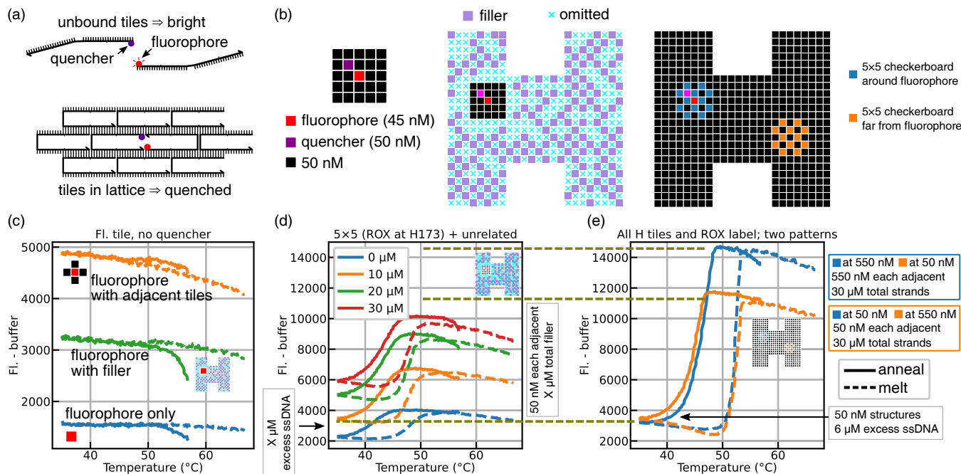
Figure 2.2: A two-tile label pair, separating the fluorophore and quencher, gives quenching from lattice growth without significant interference from intermediate states, but effects on fluorescence related to other strands complicate quantitative interpretation of fluorescence in terms of absolute tile and structure concentrations. (a) The label scheme uses two nearby tiles, along the same helices but not binding to each other directly, with one tile reversed in orientation, resulting in 5' modifications on the two tiles being constrained to be near to each other in a well-formed lattice, but not constrained in any potential complex of two or three tiles. (b) To characterize the label pair behaviour, we ran experiments with several combinations of components, based around a ROX fluorophore on tile H173 and a 5 × 5 surrounding area. A 'filler' mix included all tiles unique to H outside a 7 × 7 region around the fluorophore tile, intended to provide a mix of non-interacting tile-like DNA strands. Complete H structure samples used the same ROX fluorophore tile, with its adjacent quencher tile, and 5 × 5 area, but with one of two possible checkerboard patterns (blue or orange) of increased concentrations. (c) An anneal and melt with the (H173 with ROX) fluorophore tile and no quencher tile, including only the fluorophore tile, the fluorophore tile with 10 μM total filler concentration, and the fluorophore tile with each of the four tiles adjacent to it that each bind by one domain. We interpret the anomalously low fluorescence at the beginning of the anneal, which started by cooling from just below 60 °C, to the samples not yet having established equilibrium. (d) An anneal and melt of a 5 × 5 block with varying total concentration of filler tiles. The filler strands are expected to remain unbound at all temperatures. (e) An anneal and melt of a complete H structure, including the same label pair. At high temperature, the blue and orange samples are expected to have the same total concentration of strands, but different concentrations of tiles adjacent to the label. At low temperature, if structures have completely grown, the two samples are expected to have the same concentration of structures and of excess, unbound strands. For c-e, samples were held at 70 °C for 10 minutes, ramped to 57 °C at 1 °C/min, held at 57 °C for 20 minutes, ramped from 57 °C to 35 °C at 6 minutes per 0.2 °C, then ramped from 35 °C to 67 °C at 4 minutes per 0.2 °C. (Note that the extent of hysteresis depends on ramp speed and reflects the nucleation barrier kinetics and melting kinetics.)
