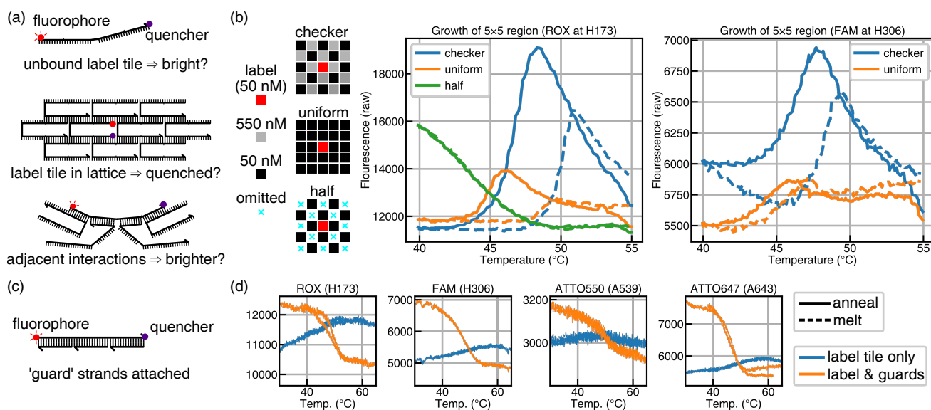
Figure 2.1: An initial design for a label tile consisting of a fluorophore and quencher on a single SST. (a) As a free unstructured strand, the fluorescence will not be fully quenched. (b) To examine the label tile’s behaviour, we used three patterns around a 5 \times 5 set of tiles from shape H, surrounding ROX on tile H173 or FAM on tile H306. The ‘checker’ pattern had high concentrations of tiles adjacent to the label tile, while the ‘half’ pattern omitted a checkerboard pattern of tiles such that the full 5 \times 5 structure could not form. An anneal and melt of the patterns around a ROX label tile and FAM label tile shows a significant increase in fluorescence during the anneal. (d) To examine whether DNA binding to the label tile ‘stretched’ the strand, reducing self-quenching, we used ‘guard’ strands that each bound to a third of the tile. (e) For all four fluorophores, samples with guard strands showed a significant increase in fluorescence during the anneal around 50^\circ\text{C} .
