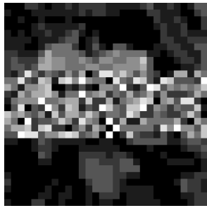
Nucleation model: ObscMagn2
