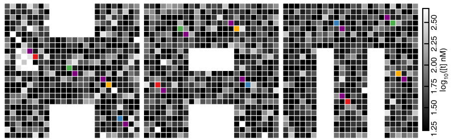
Per-tile nucleation rate: ObscHazeln3, G_{se}=5.6 , trials=40000
