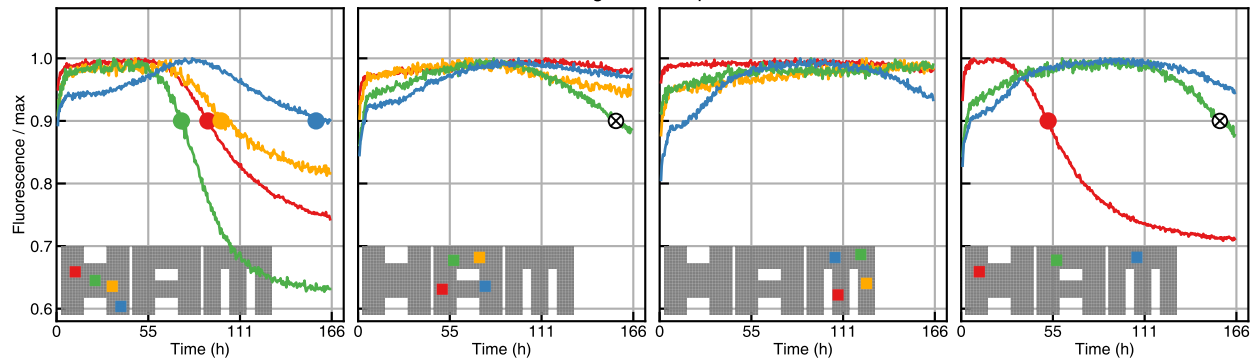
Pattern recognition ramp: Harom
