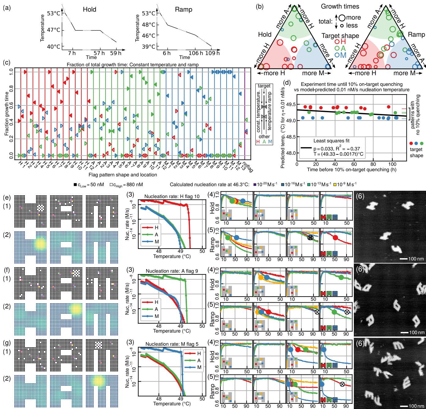
Fig. E6 | Nucleation and growth with 'flag' patterns of enhanced concentration. a–c, 37 different concentration patterns with enhanced concentrations of shared tiles in 5 \times 5 regions were prepared, each with four different standard sets of fluorophores in four samples, and grown using two temperature protocols (a): a ramp focusing on 48°C to 46°C over 100 hours, and a hold at 47°C. Using growth times as described in Extended Data Fig. E5, fluorescence data for many samples in both experiments showed preference for the desired shapes (b, c), but with considerable variation in selectivity and total amount of growth. d, No statistically significant correlation was found between the nucleation model prediction for temperature of on-target nucleation and the time of on-target shape quenching in the temperature ramp experiment. Although the nucleation model overestimates the nucleation temperature and its nucleation rate estimates may be far off, our interest here is in the qualitative features and difference between the shapes. e–g, Details of three patterns, with concentration patterns (1), weighted critical nucleus free energy starting from particular tiles (2), nucleation-model-estimated nucleation rates (3), temperature hold (4) and temperature ramp (5) experiment fluorescence results, and (6) AFM images from the temperature hold experiments. Information for all individual flag patterns is available in the Supplementary Information and Data Appendix, Section 5 .
