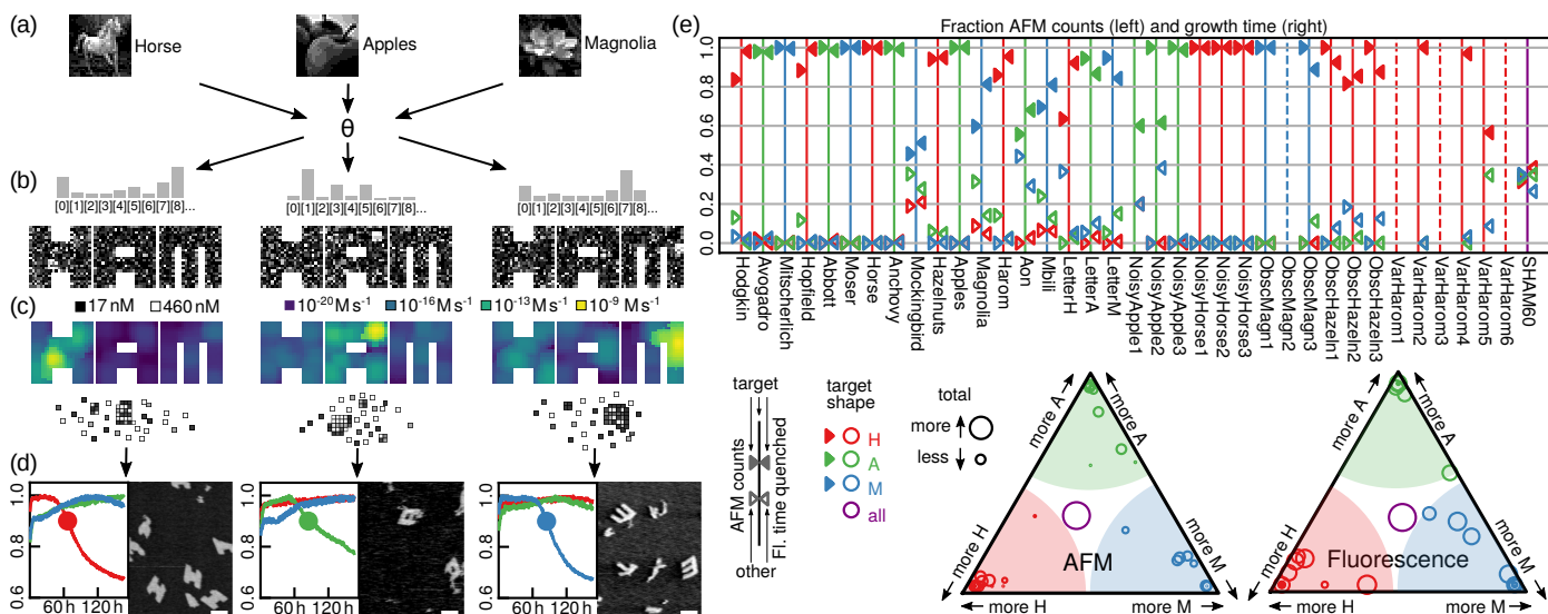
Fig. 6 | Pattern recognition results with a pre-existing multifarious system. a–c, All images (three shown) are converted (a) through a single pixel-to-tile map \theta to vectors of tile concentrations (b), which are shown mapped onto tile locations in each shape, with nucleation rate predictions (c). d, Normalized fluorescence over time in hours (one label per shape; other label configurations shown in Extended Data Fig. E9) during a 150 hour temperature ramp from 48 °C to 45 °C, and final AFM images (with 100 nm scale bars). e, Summary of results for both fluorescence and AFM for all 36 images, and a uniform 60 nM tile concentration control sample. Above, colors of vertical lines indicate the target shape for each pattern, while triangular markings of each color indicate the relative fraction of growth time (on right) or fraction of shapes counted in AFM images (on left) for the corresponding shape (solid markings indicate target shape). Dashed lines indicate samples with no significant quenching or observed shapes. Below, ternary plots summarize the same results, with proximity to triangle corners indicating relative fractions of growth time (right) or counted shapes (left), and circle size indicating overall growth time (right) or total number of shapes (left).
