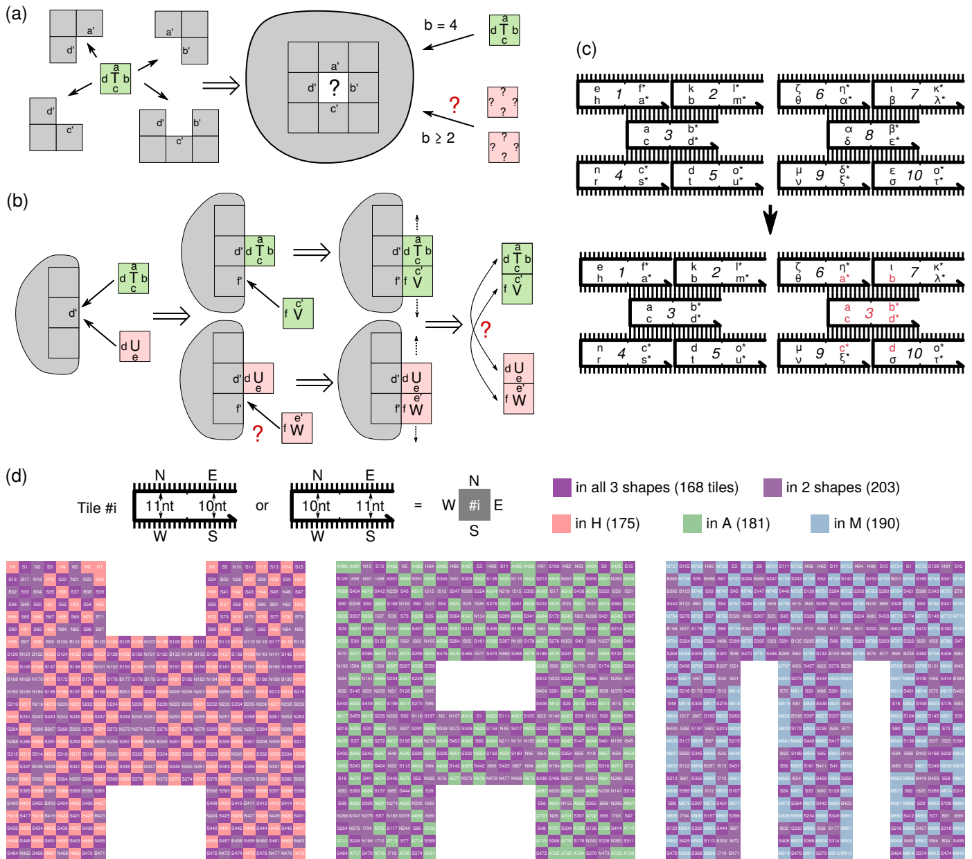
Fig. E2 | Proofreading tile set design and tile assignment map. Extensive promiscuous interactions present in the SHAM mix could in principle lead to unintended chimeric structures and other malformed assemblies. To reduce or prevent such behaviors, our design incorporates self-assembly proofreading principles, so called because they enhance quick rejection of mis-assembled tiles. Much like with neural networks, 67 random arrangement of tiles (such as the initial checkerboard layout in the first stage of our design process) provides a statistical proofreading 23 in the sense that problematic interactions are unlikely to arise. Further optimization of the tile set (in our second stage) ensures that two types of problematic interactions do not occur, thereby conferring algorithmic proofreading 35 and self-healing properties. 58 This tile set optimization is derived from prior work. 36 a , Our systems are designed to grow in a regime where a tile attaching by at least two bonds is favorable, but a tile attaching by one bond is not ("threshold 2"). Motivated by self-healing tile systems, 58 we seek a tile set where no correct partial assembly should ever allow an undesired tile to attach by two or more bonds, though undesired attachments by one bond are allowed, such that any favorable attachment to a partial assembly will be correct. b , In addition to tiles attaching favorably by 2 bonds to growing facets, new facets in the system will only be created by tiles attaching unfavorably by one bond, and then being stabilized by further, favorable growth. At a site where tile T would correctly attach by one bond, a tile U might be able to attach incorrectly by the same bond. T would correctly be stabilized by the subsequent attachment of V by two bonds, but U might be stabilized as well if there is a tile W that can attach to it and shares the same glue. Thus, if for every pair of tiles that can bind to each other (e.g., T + V ), there is no other pair of binding tiles (e.g., U + W ) that share two glues on the same edges of the tiles, then any tile that attaches by one bond to an assembly will either be the correct tile, or will not allow a subsequent stable attachment, and will likely detach quickly. This is equivalent to 'second-order sensitivity' with all directions treated as inputs, functioning as a form of self-assembly proofreading. 35,36 c , We created a multifarious tile system by first starting with three shapes constructed entirely of unique tiles, then repeatedly attempting to 'merge' tiles in different shapes by constraining the sequences of their domains to be identical, and checking whether each merge of two tiles results in a tile system that does not have any tile pairs violating criteria in a and b . d , From multiple trials of the merging process, each initially favoring a checkerboard arrangement before attempting more general merges, we selected the smallest result containing 917 tiles. DNA sequences for tiles in the system were designed with the single-stranded tile (SST) motif, 31 with two alternating tiles motifs of 10 nt and 11 nt domains (full shape layouts and tile sequences are shown in Supplementary Information and Data Appendix, Sections 3.3 and 4.1 ).
