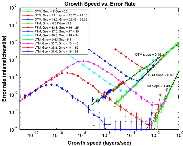
Fig. 14 Growth speed versus error rate. Self-assembly of 1,000,000–50,000,000 tiles represent one point. The error rate is given as 10^{-7} if the simulation results in no errors. Error bars of these plots show two standard deviations: \sigma = \sqrt{\epsilon}/\sqrt{m} where m is the total number of tiles grown in all simulation runs under a given G_{se} and G_{mc} and \epsilon is the total number of mismatches divided by the total number of tiles. Red, blue, magenta, and light blue curves show each run at varying concentrations under fixed temperature (i.e., fixed G_{se} ). Green plots show simulations along estimated Pareto-optimal boundaries for each mechanism, and black lines show their approximations
