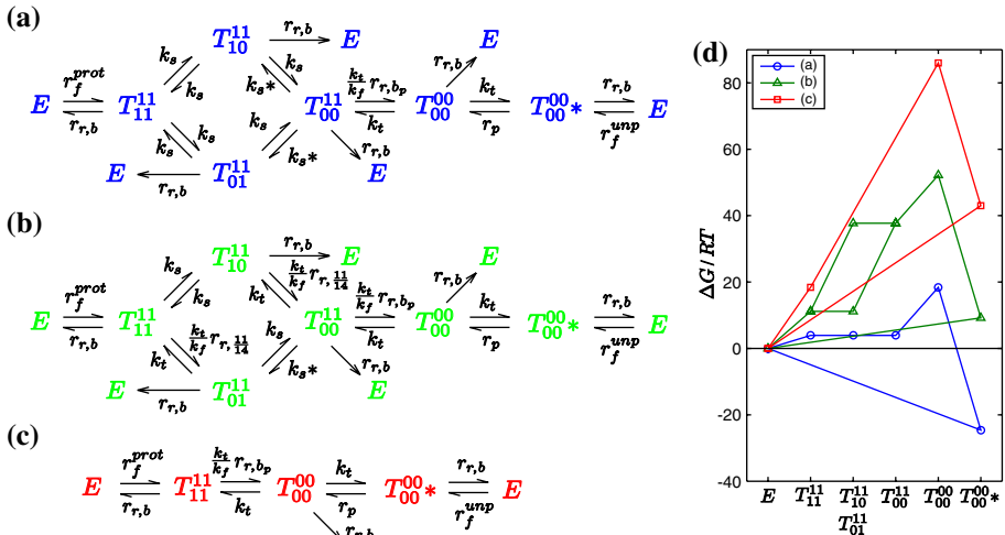
Fig. 10 Markov process for the LTM in cases of a tile matching by (a) two inputs, (b) one input (e.g., the right input), and (c) neither input. Each diagram has seven states ( E, T_{11}^{11}, T_{10}^{11}, T_{01}^{11}, T_{00}^{11}, T_{00}^{00} and T_{00}^{00*} ). Subscript and superscript of T represent whether the input and output sticky ends of the protection tile are detached from (0) or attached to (1) the foundation tile. (d) The relative free energies of the substate at each case when \tau = G_{mc}/G_{se} = 18.4/33.8 \approx 0.54
