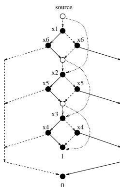
Figure 2.5: Implementing a function using a nondeterministic branching program. f(x) = “\mathbf{x} is palindromic except for isolated (non-adjacent) errors”. NBP(f) \leq 2n + 2 .
