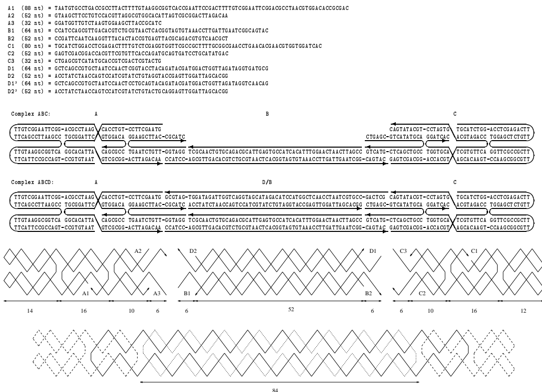
Figure 4.1: Sequences and Structures for ABCD. Sequences are written 5' to 3'. 3' ends are denoted by arrows in the diagrams, and strand labels are near 5' ends. Lengths are measured in nucleotides. Above, sequence details are given along with schematic representations of ABC and ABCD (not ligated). Below, more geometric detail is sketched for A, B, C, D, and ABCD (ligated). Diagrams illustrate intended structures only.
