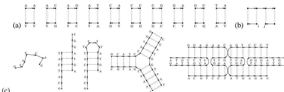
Figure 3.9: Some DNA complexes. Solid lines represent backbone edges; each dotted line represents a pair of reciprocal basepair edges. (a) The 10 Watson-Crick subgraphs. (b) The valid ligation site. (c) A strand, a duplex with sticky ends, a hairpin with a sticky end, a 3-armed branched junction, and a DAO double crossover (DX) unit with sticky ends.
