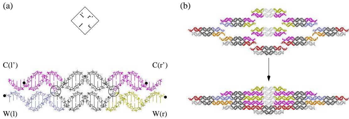
Figure 3.21: The DNA representation of Wang tiles. (a) A molecular Wang tile (double crossover molecule) representing the rule (l, r) \rightarrow (l', r') . The molecule consists of an interior structural region and four double-stranded arms, each terminated by a single-stranded sticky end. Edge labels are implemented using unique sticky-end sequences. Note that sticky-ends for the lower edges use Watson-sense sequences for each label, while the upper edges use the complementary Crick-sense sequences. This ensures the proper relative orientation of tiles. As shown, the same molecule represents both a Wang tile and its reflection about the vertical axis; however, using four encodings for each label ( W_{left}, W_{right}, C_{left}, C_{right} ) eliminates reflection-sense binding. In the double crossover molecule, the crossover points are circled, and dots are placed at the 5' ends of each strand. Color is used to indicate the edge label being represented, and not the identity of strands (each strand is multi-colored). (b) The self-assembly of 9 molecular Wang tiles, of 5 distinct types. These correspond to the 9 tiles at the bottom of Figure 3.19c. Note that the corner and boundary molecules have hairpin sequences, and thus no sticky ends, on certain of their lower arms; this implements a tile with strength-0 labels on its lower edges. Also note that on the corner and boundary molecules, the red and orange sticky ends are sufficiently longer than the sticky ends on the rule molecules to implement a strength-2 interaction.
