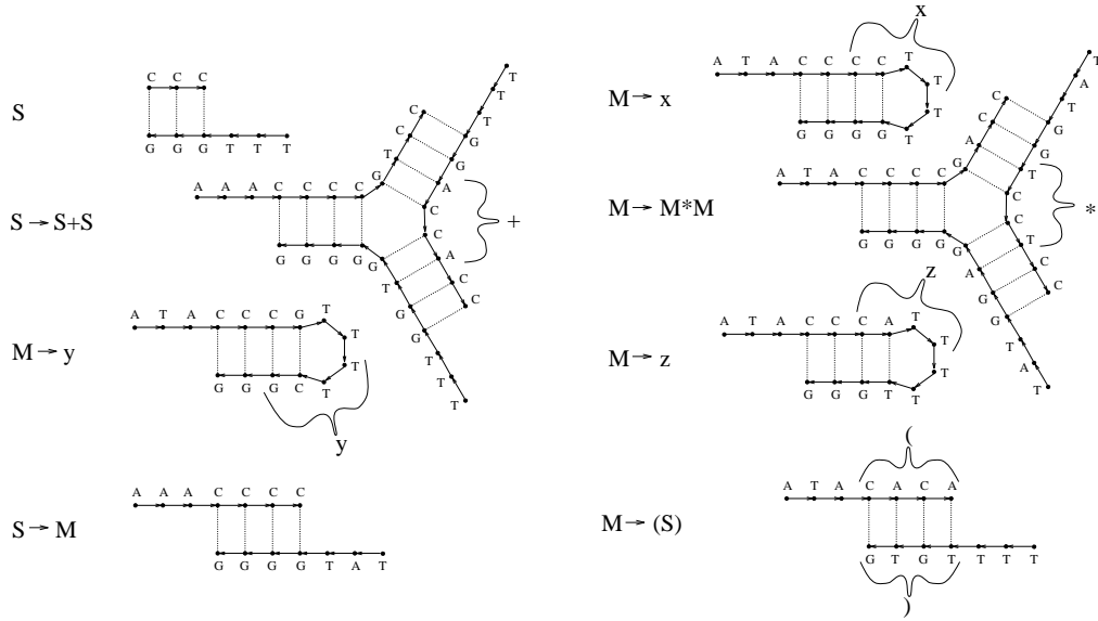
Figure 3.12: The initial complexes A corresponding to the regular grammar G_F . The codebook \mathcal{C} defines \mathcal{C}_x = CCTT , \mathcal{C}_y = TTCC , \mathcal{C}_z = CATT , \mathcal{C}_\cup = CACA , \mathcal{C}_\cap = TGTG , \mathcal{C}_+ = ACCA , and \mathcal{C}_* = TCCT . We use R_1^3 .
